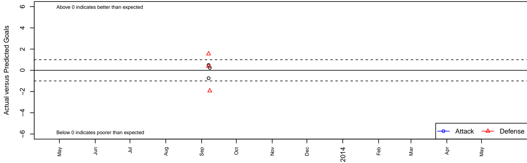
Flathead Force G99 Dots are actual minus expected GF (blue circles) and GA (red triangles). Blue line is smoothed change in attack strength. Red is smoothed change in defense strength.
